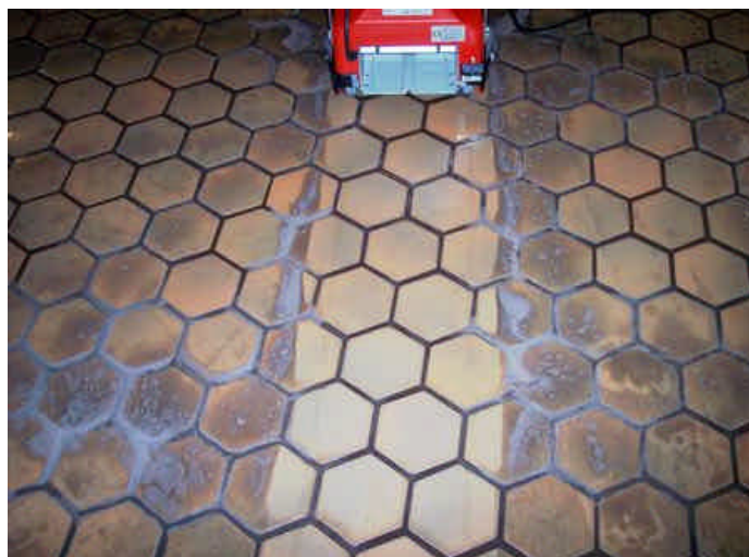
The Turbolava two counter-rotating brushes scrub the floor and allows the same equipment to extract the soil into a recovery tank
